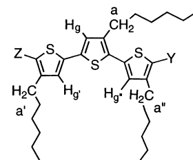
Figure 3. Detailed structure of polymer showing significant protons for NMR characterization.
