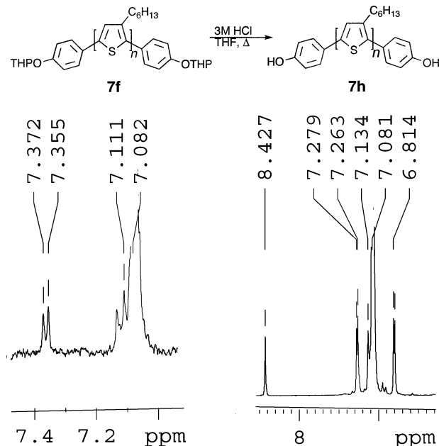
Figure 5. Aromatic region of 1 H NMR spectra of tetrahydropyranyl and phenol terminated polymer.
